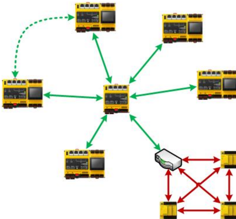
Figure 4 Hub and spoke topology of BACnet/SC. While the BACnet/SC communication is centralised in the hub, the BACnet/IP communication is station to station or broadcast.
